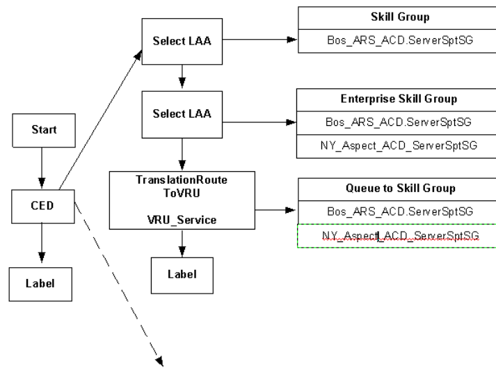
Figure 12: Sample Script for Hybrid Routing
