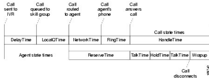
Figure 13: Agent State and Task State Relationship
