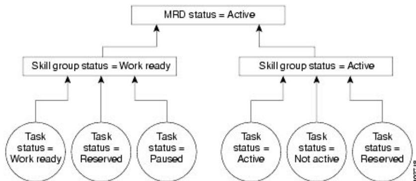
Figure 18: Agent State Hierarchy
